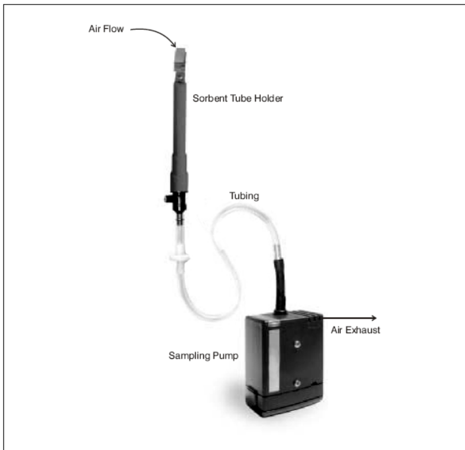
Figure 6-8 Example Sampling Pump for Mercury Sampling Using a Sorbent Tube
