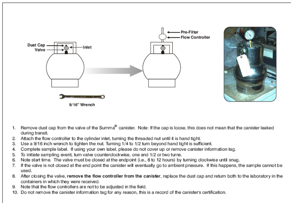
Figure 6-7 VOC Sampling Using a Summa® Canister
