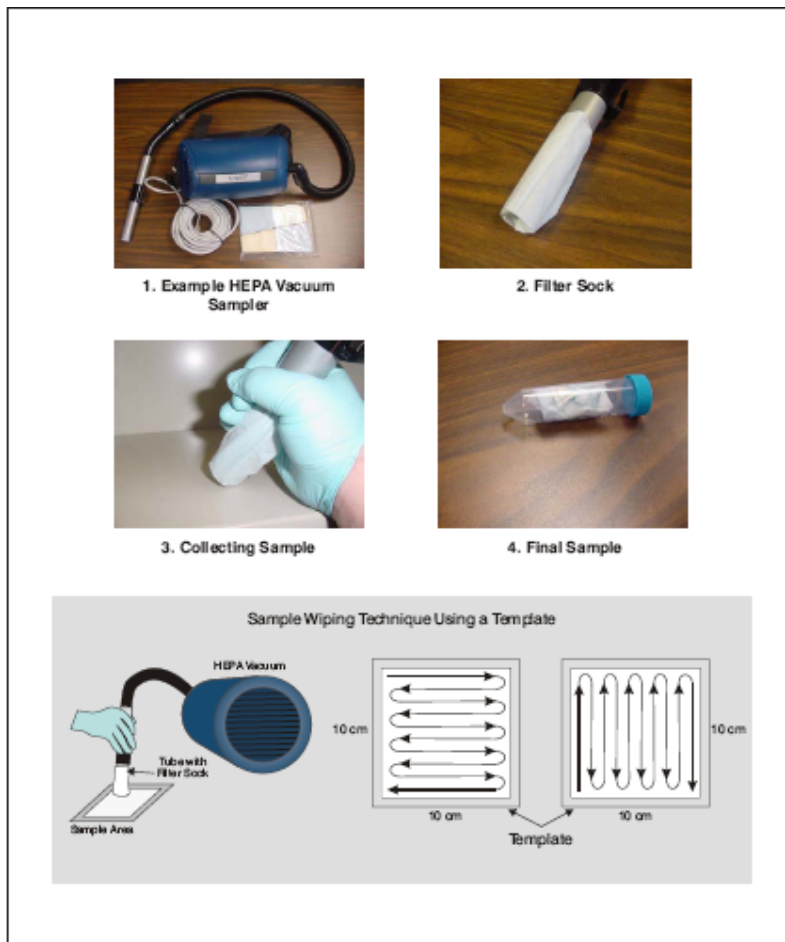
Figure 6-6 HEPA Vacuum Sampling Illustration
