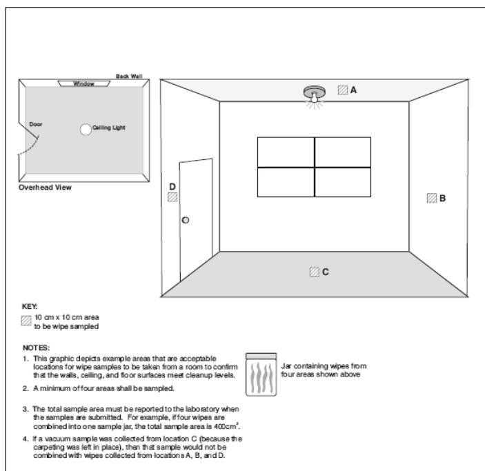
Figure 6-3 Example Ceiling, Floor, and Wall Sampling Locations for Composite Wipe Samples for Methamphetamine and/or Lead
