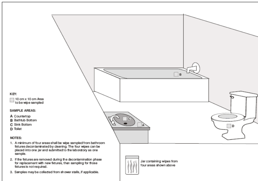
Figure 6-5 Example Bathroom Sampling Locations for Composite Wipe Samples for Methamphetamine and/or Lead
